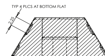
SECTION E-E SECT E-E SHOWING RECESS POCKET DETAIL FOR REFLECTIVE TAPE
