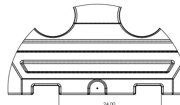
DETAIL D SCALE 1 : 6 REV 2 SHOWING TRUE CENTER TO CENTER DIMENSIONS OF FORK THRU-HOLES
